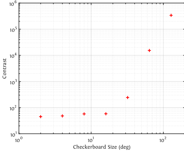
Figure 16: HDR VR display contrast measurement. The contrast ( y -axis) of our HDR VR prototype were measured for increasing checkerboard size ( x -axis). Both axes are plotted on a log scale.
