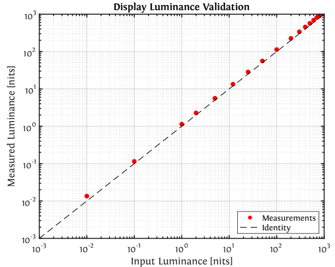
Figure 13: Additional haploscope calibration results. A Spectrascan PR-745 was used to measure luminance patches rendered in PsychToolbox. The x -axis is the input patch luminance, and the y -axis is the luminance measured by the PR-745 (both on a log-nit scale). Red points are measurements, and the dashed line is identity.
