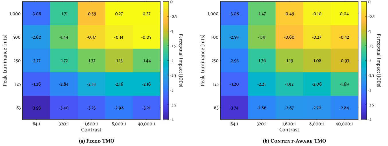
Figure 11: Complete user study results. Results of the main user study are plotted here for both the (a) FIXED TMO and the (b) CONTENT-AWARE TMO. Colors represent JOD values (defined in the color bar), with values labeled in each cell of the matrix. x -axis represents contrast, and y -axis peak luminance (nits). Here, the reference condition (not shown in these plots) was mapped to 0 JODs.
